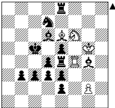
h#3 3 solution
