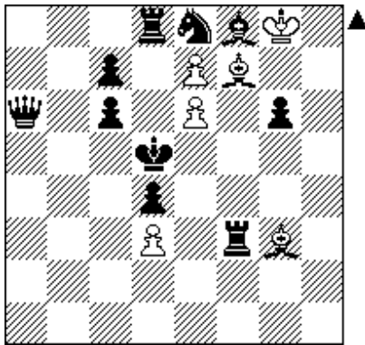
h#2 3 solution
